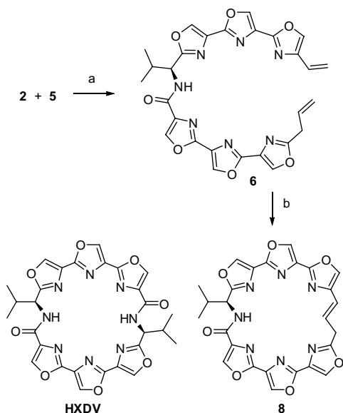
Scheme 3. Reagents and conditions: (a) EDC, HOBT, DMF, 0 °C to rt, 69%; (b) 7b , CH 2 Cl 2 , Δ, 96 h, 32%. Structure of HXDV shown for comparison.
