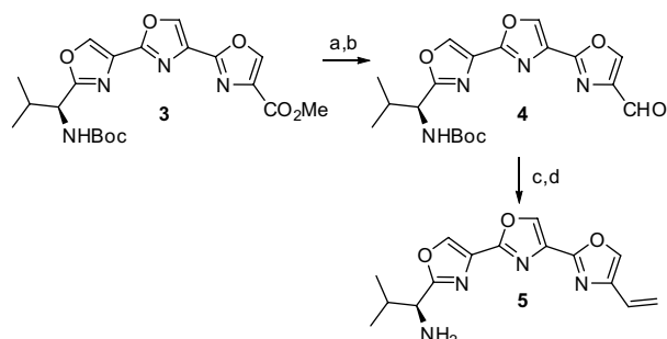
Scheme 2. Reagents and conditions: (a) NaBH 4 , LiCl, THF/MeOH (1:1) 73 %; (b) oxalyl chloride, DMSO, CH 2 Cl 2 , Et 3 N, –78 °C, 88%; (c) Ph 3 PCH 3 Br, n -BuLi, THF, 0 °C to rt, 74%; (d) TFA, CH 2 Cl 2 , 0 °C, 73%.
