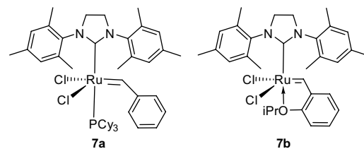
Figure 1. Metal carbene catalysts employed in this study.
