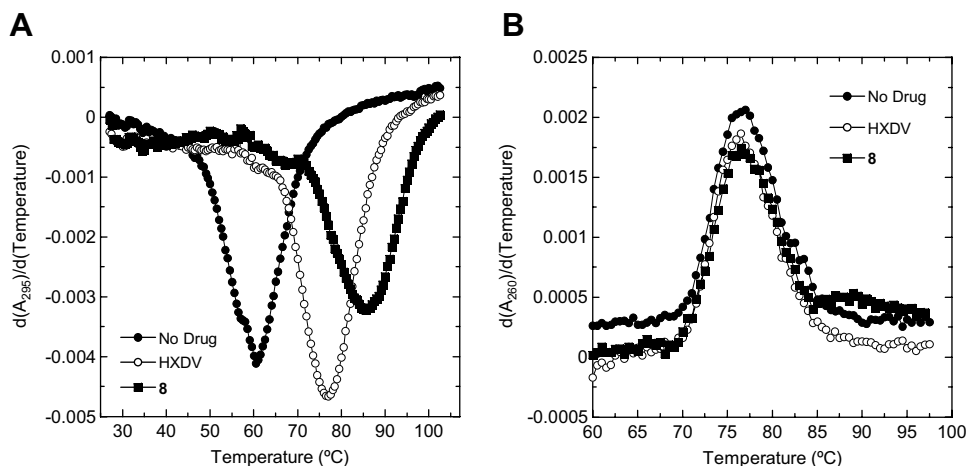
Figure 2. First-derivatives of the UV melting profiles of d[T 2 G 3 (T 2 AG 3 ) 3 A] (A) and ST-DNA (B) in the absence and presence of HXDV or compound 8 . Profiles were acquired on an AVIV model 14NT-UV-vis spectrophotometer using quartz cuvettes with a 1 cm pathlength. The temperature was raised in 0.5 °C increments and the samples were allowed to equilibrate for 1.5 min at each temperature setting, whereupon absorbances were recorded over a period of 5 s and averaged. When present, ST-DNA was used at a base pair concentration of 15 μM, while d[T 2 G 3 (T 2 AG 3 ) 3 A] was used at a strand concentration of 4 μM. Macrocylic ligands were used at a concentration of 15 μM in the ST-DNA experiments and 20 μM in the d[T 2 G 3 (T 2 AG 3 ) 3 A] experiments. The solution conditions were 10 mM EPPS (pH 7.5) and sufficient KCl to bring the total K + concentration to 50 mM. In the ST-DNA experiments, the acquisition wavelength was 260 nm, while being 295 nm in the d[T 2 G 3 (T 2 AG 3 ) 3 A] experiments.
